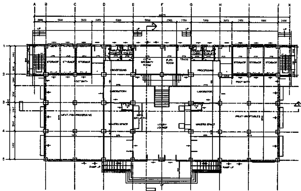
TESDA INNOVATION CENTER - ISAT A' GROUND FLOOR PLAN SCALE: 1:2000/13
