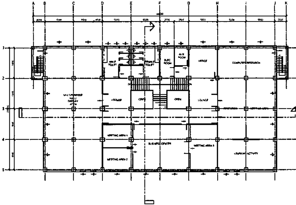
TESLA INNOVATION CENTER - ISAT A SECOND FLOOR PLAN SCALE 1/32"=1'-0"
