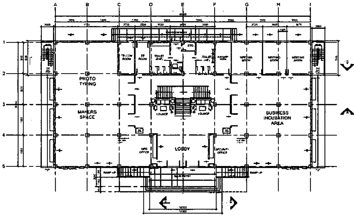
TESDA INNOVATION CENTER - MARIVELES A GROUND FLOOR PLAN SCALE 1:200MMS
