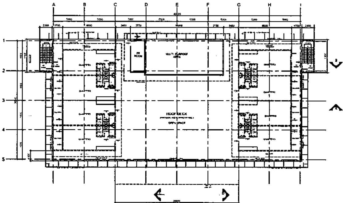
TESDA INNOVATION CENTER - MARIVELES ROOF DECK PLAN SCALE 1:200MTC
